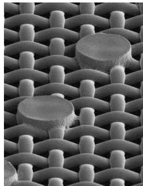
Stencil adhesion of SEFAR® PET 1500 120/305-34Y
